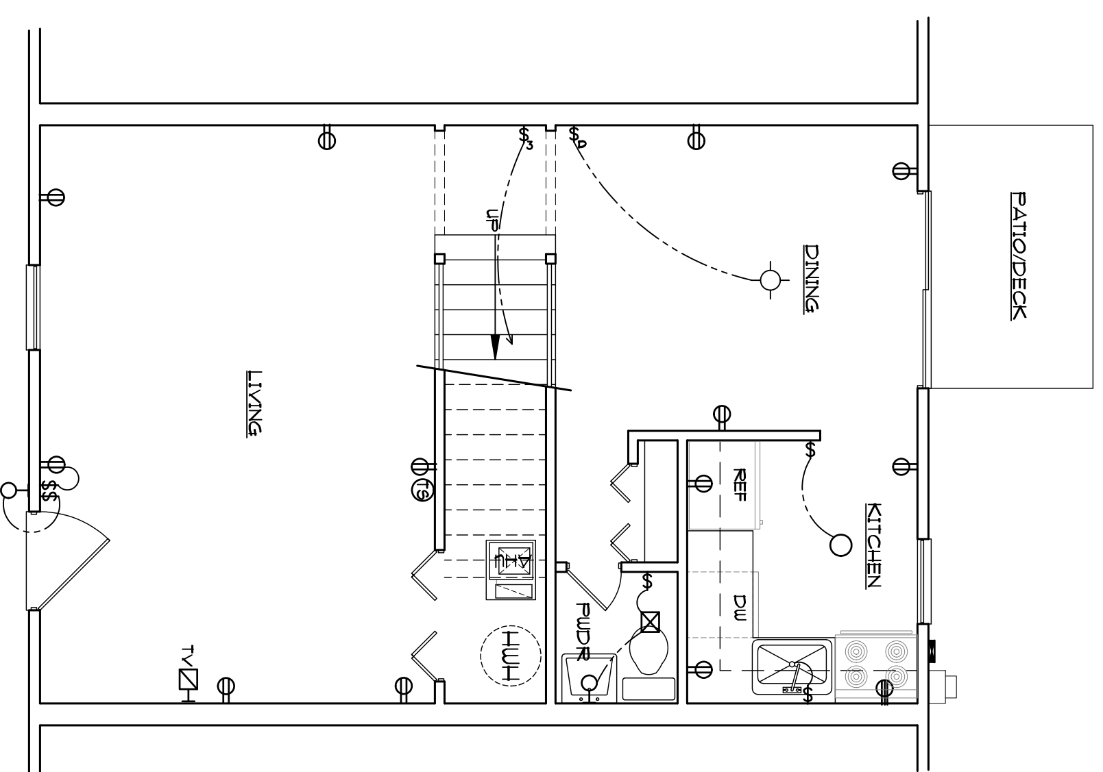
1 MAIN FLOOR
